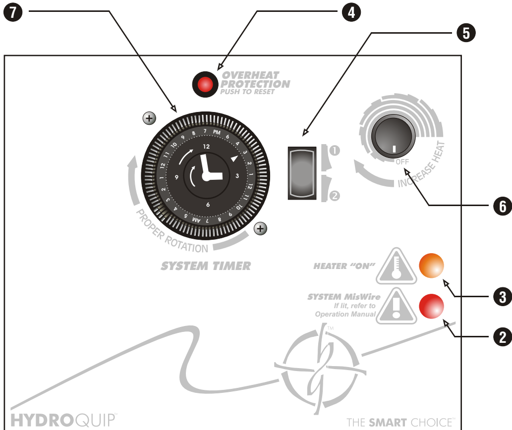
FRONT PANEL
